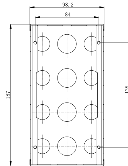
1 FRONT VIEW
