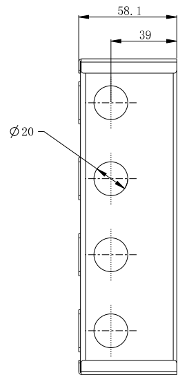
2 RIGHT VIEW
